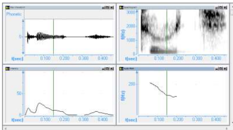
Graph 2: [t̀̀:c] 162.8Hz
